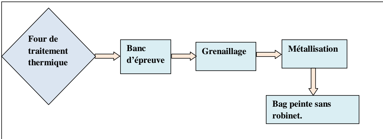
Fig.VI.4 Processus Finition
