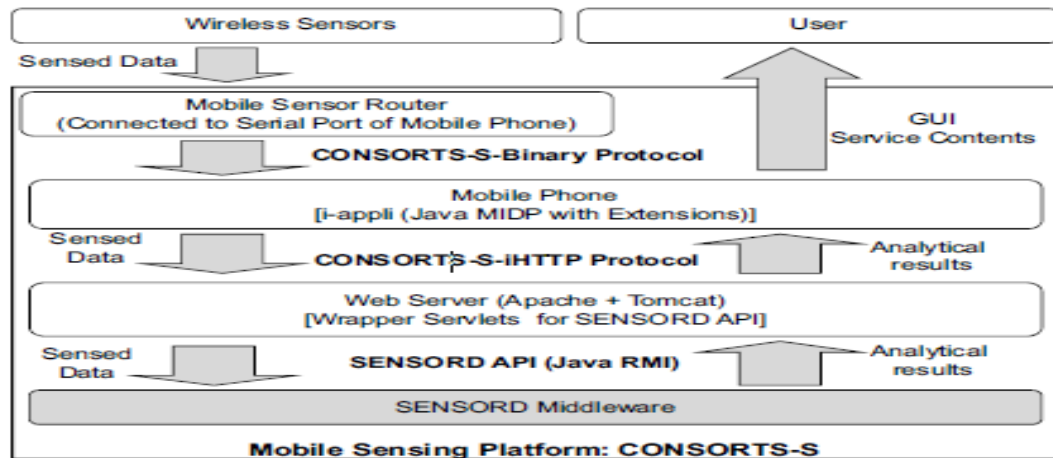
Figure IV-4 Architecture de CONSORTS-S Platform.
